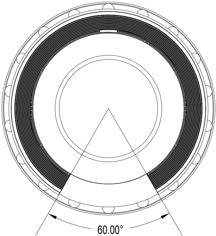
Second Position Casing Hanger (HT-HL) for the SS-15 RLD Model
